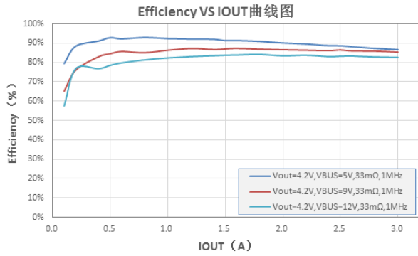
图 9 Charger Efficiency vs. I_{OUT}
