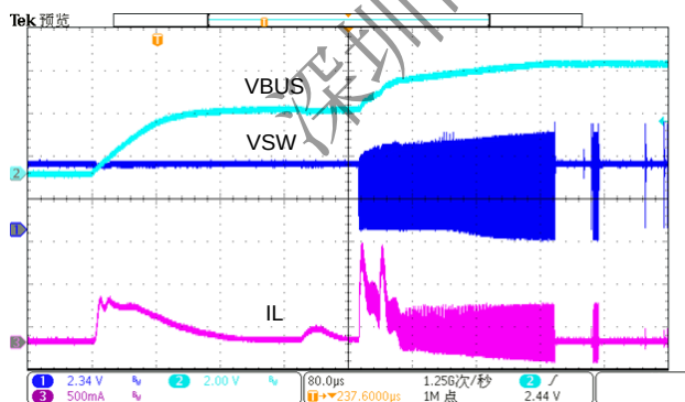
图 13 OTG 模式, Startup, 3.6V V_{BAT} , 440ohm load, additional 10uF X5R across VBUS
