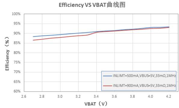
图 10 charger Efficiency vs. V_{BAT} , I_{(IN\_LIMIT)}=0.5A
