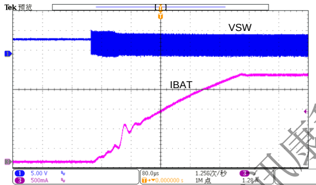
图 5 V_{\text{BUS}}=5\text{V} , V_{\text{BAT}}=3.8\text{V} , I_{\text{O(CHAARGE)}}=2.16\text{A} , No input current limit, Charge Current Ramp Up
