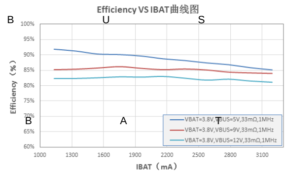
图 8 Charger Efficiency vs. I_{\text{BAT}} (WCSP Package)
